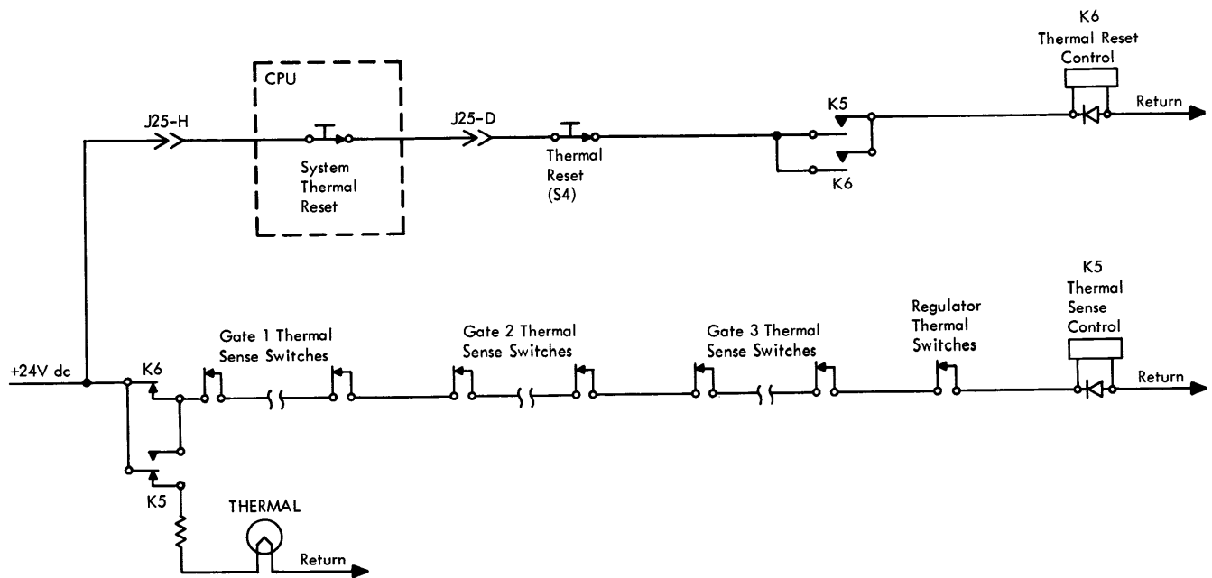
Figure 5-6. Thermal Protection Circuits
