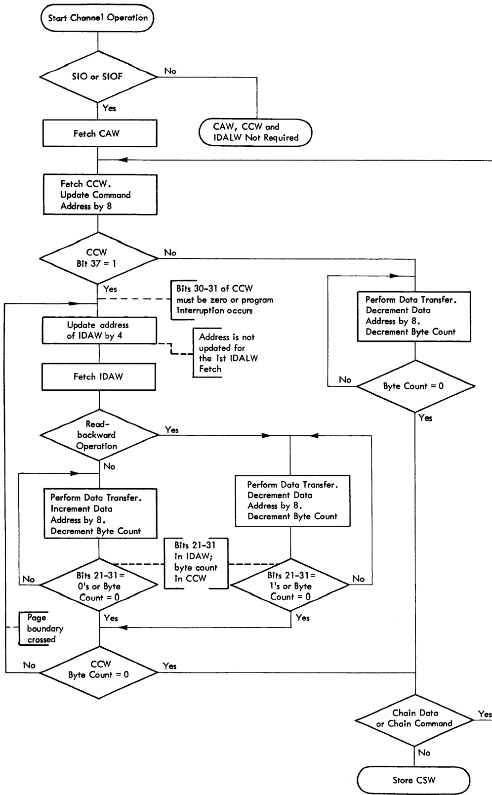
Figure 4-13. IDA Flowchart
