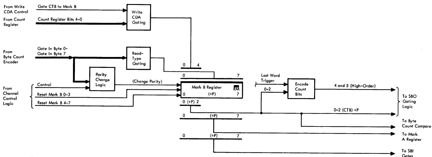
Figure 2-27. Mark-B Register, Block Diagram
