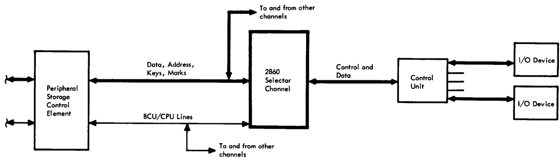
c. Selector Channel System Configuration for Model 91.
