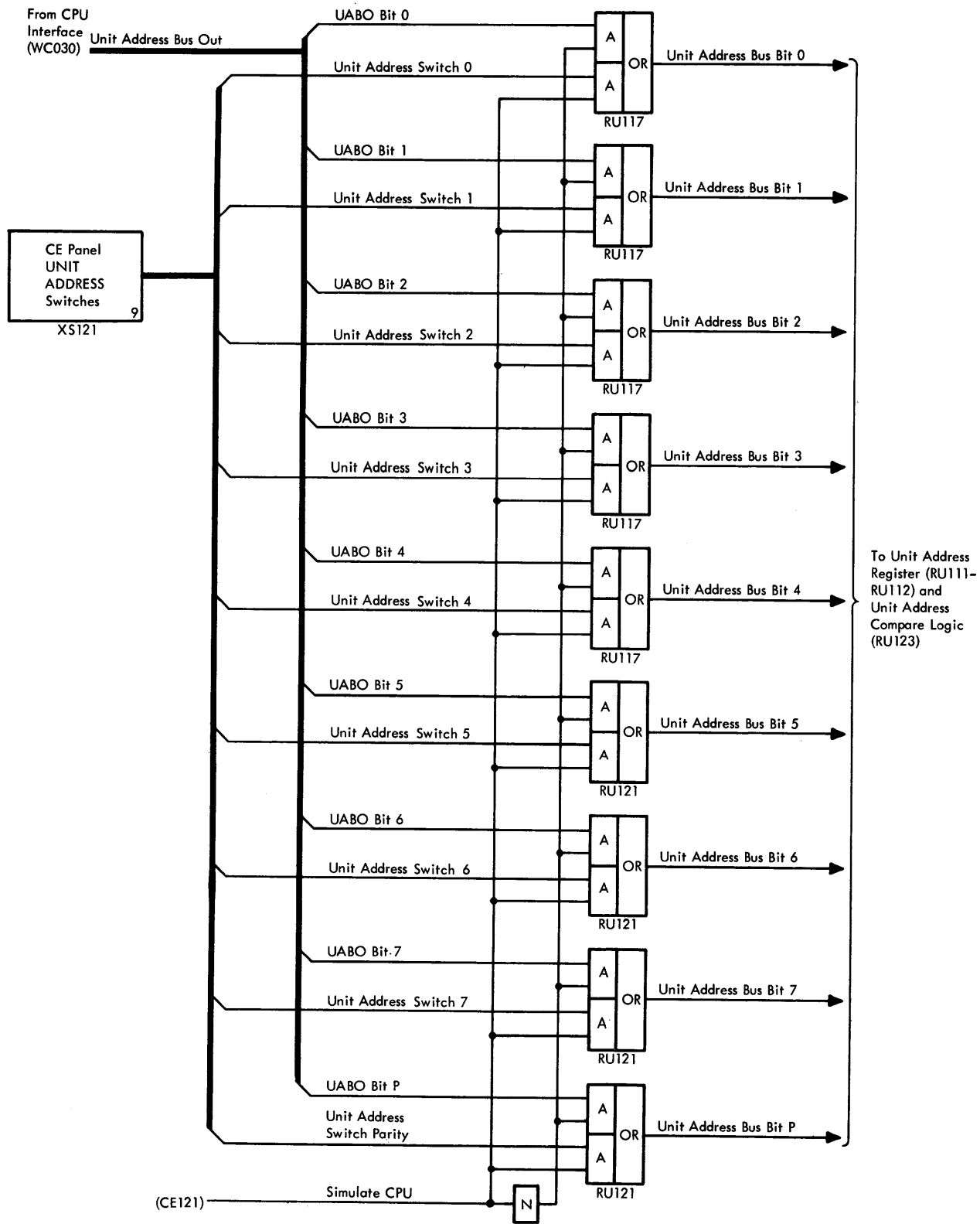
Figure 2-23. Unit Address Bus-Out Logic
