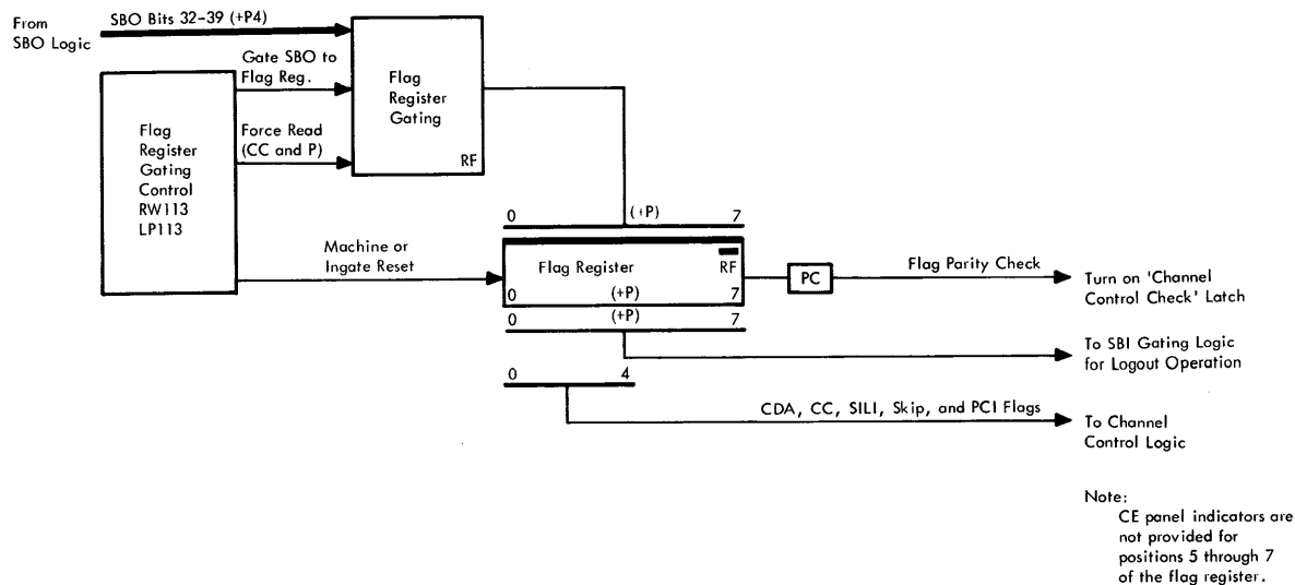
Figure 2-13. Flag Register, Block Diagram
