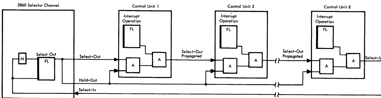
Figure 3-1. Channel Polling
