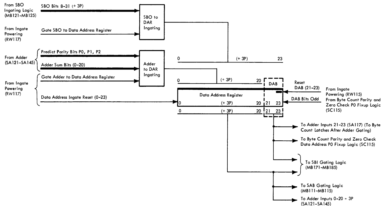
Figure 2-12. Data Address Register, Block Diagram
