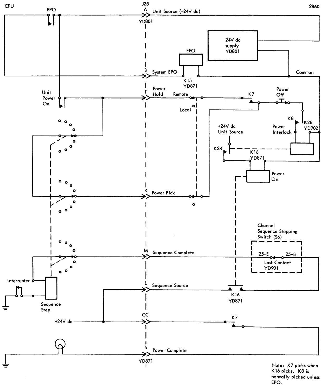
Figure 5-3. 2860/CPU Power Interface
